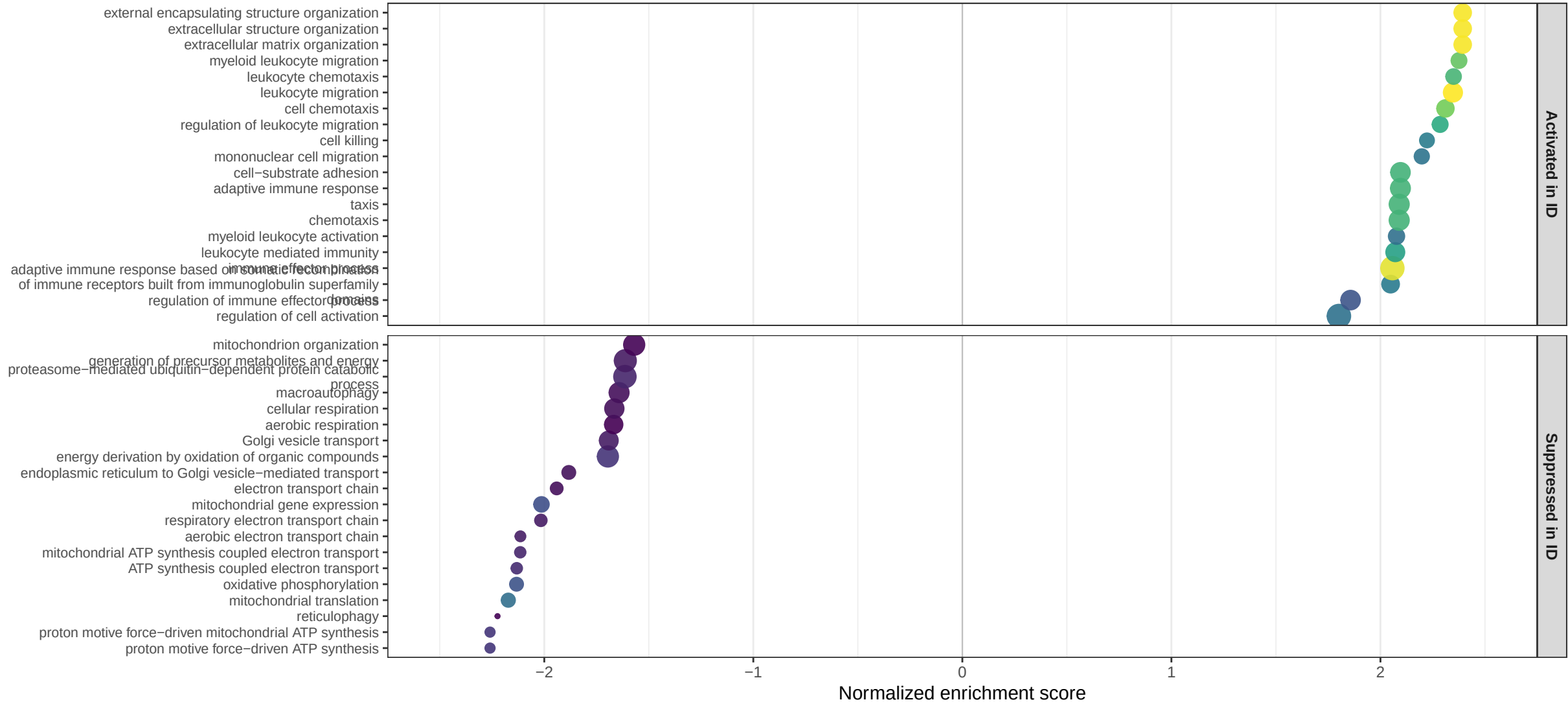
GO BP GSEA ranked by stat
