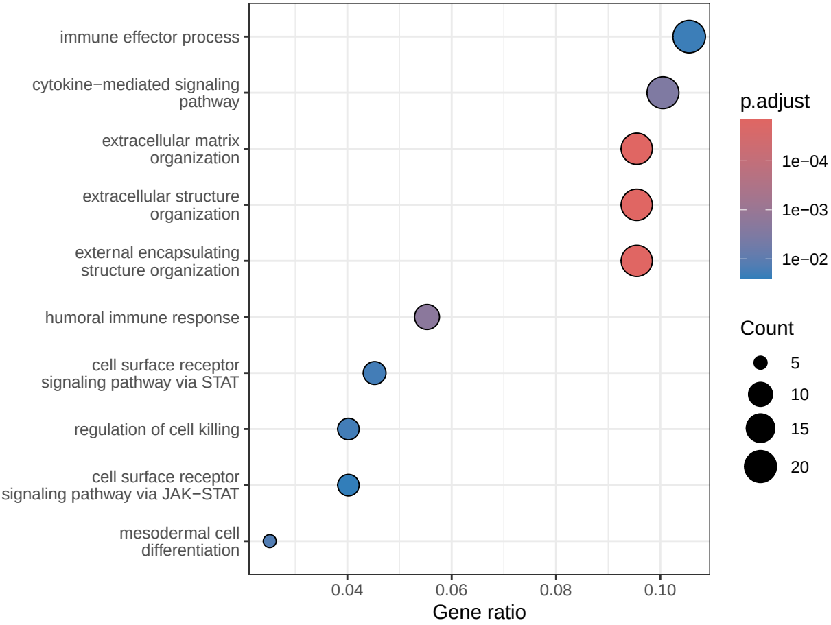
GO BP ORA: upregulated in ID
